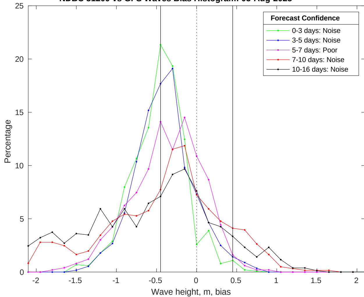
NDBC 51209 vs GFS Waves Bias Histogram: 05-Aug-2025
