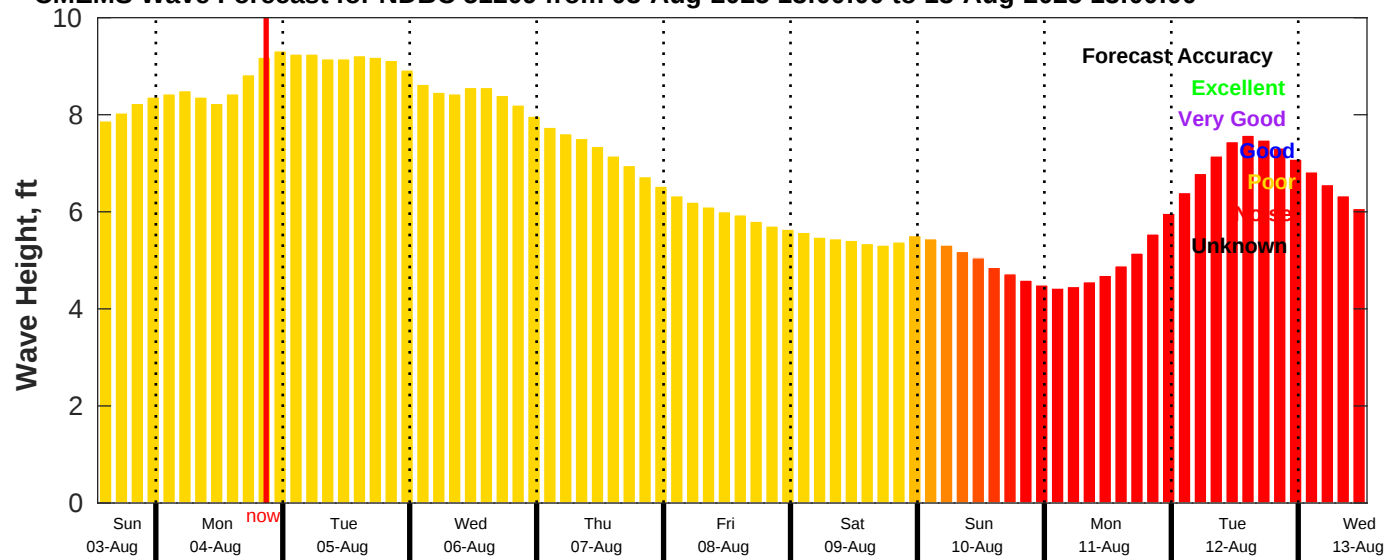
CMEMS Wave Forecast for NDBC 51209 from 03-Aug-2025 13:00:00 to 13-Aug-2025 13:00:00
