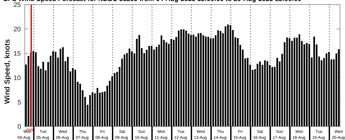
GFS Wind Speed Forecast for NDBC 51209 from 04-Aug-2025 13:00:00 to 20-Aug-2025 13:00:00
