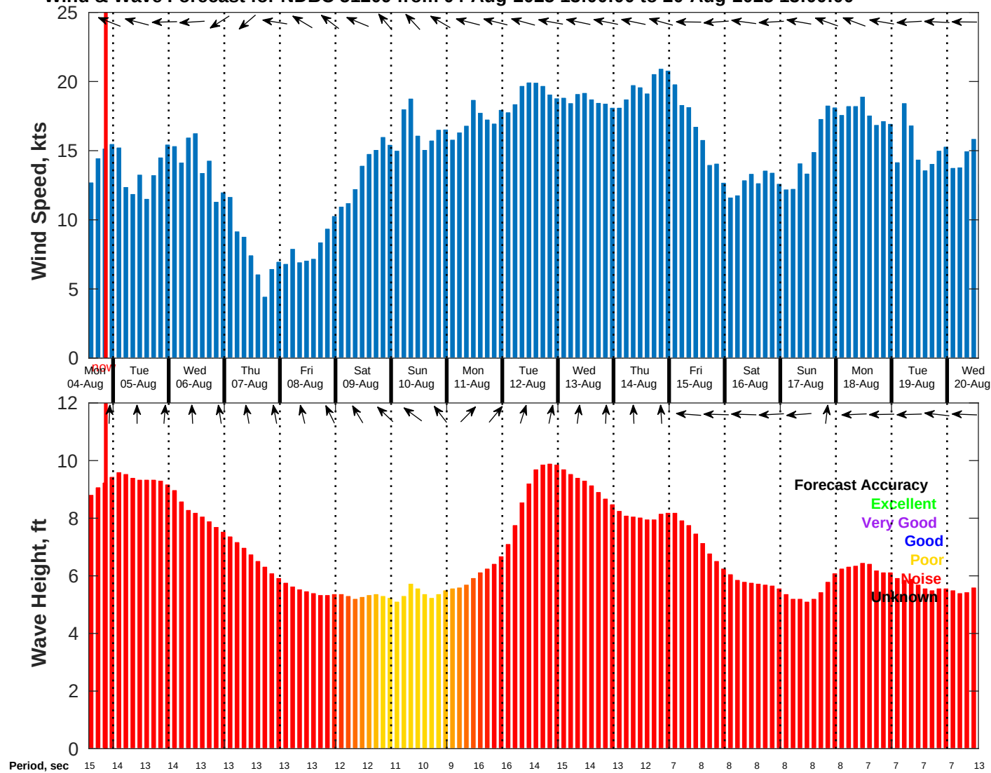
Wind & Wave Forecast for NDBC 51209 from 04-Aug-2025 13:00:00 to 20-Aug-2025 13:00:00
