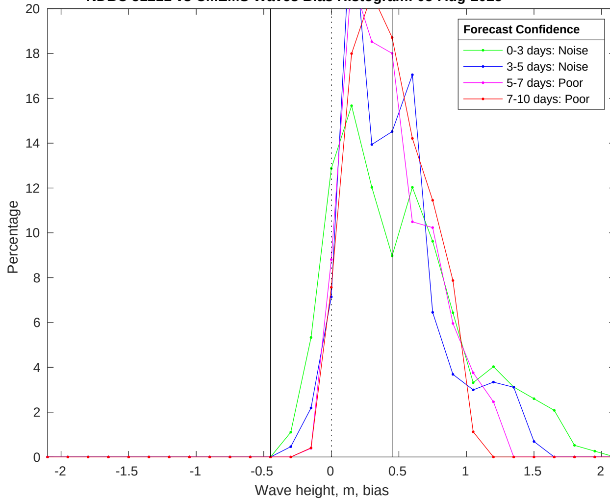
NDBC 51211 vs CMEMS Waves Bias Histogram: 05-Aug-2025
