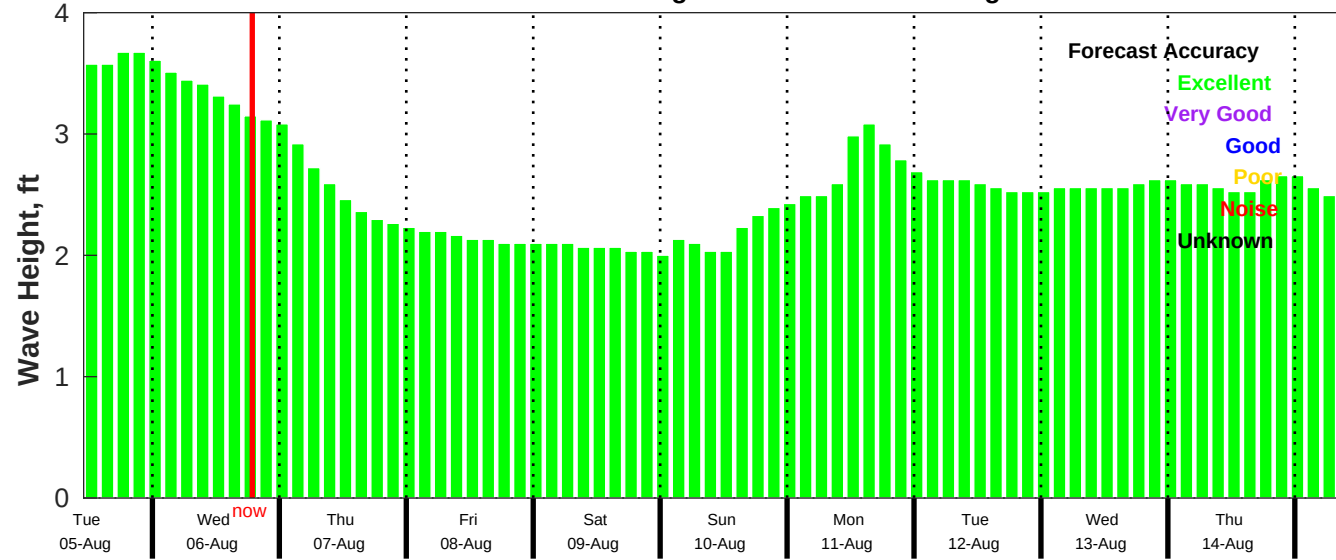
CMEMS Wave Forecast for NDBC 52211 from 04-Aug-2025 11:00:00 to 14-Aug-2025 11:00:00
