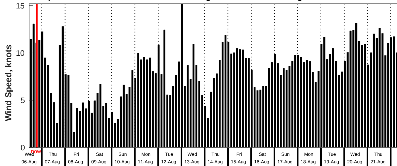
GFS Wind Speed Forecast for NDBC 52211 from 05-Aug-2025 11:00:00 to 21-Aug-2025 11:00:00
