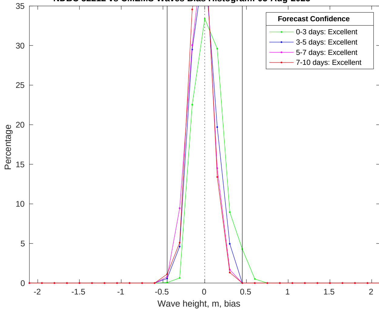
NDBC 52212 vs CMEMS Waves Bias Histogram: 05-Aug-2025
