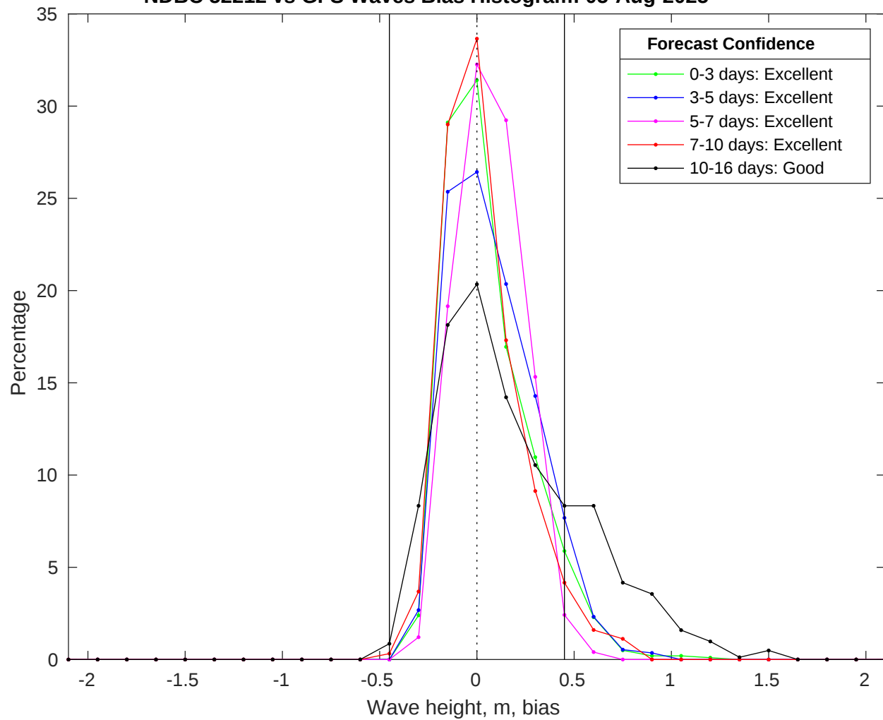
NDBC 52212 vs GFS Waves Bias Histogram: 05-Aug-2025
