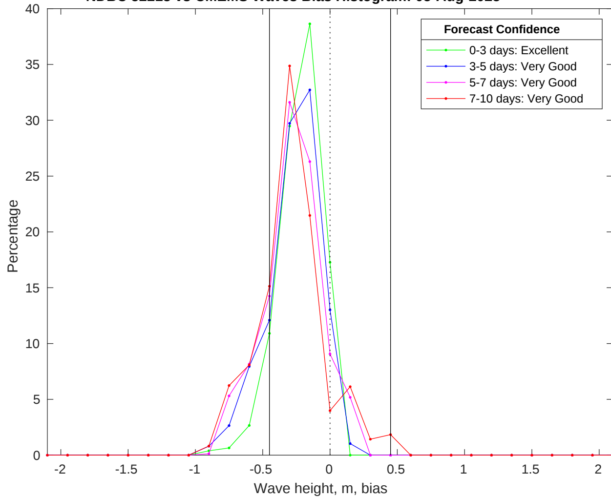
NDBC 52213 vs CMEMS Waves Bias Histogram: 05-Aug-2025
