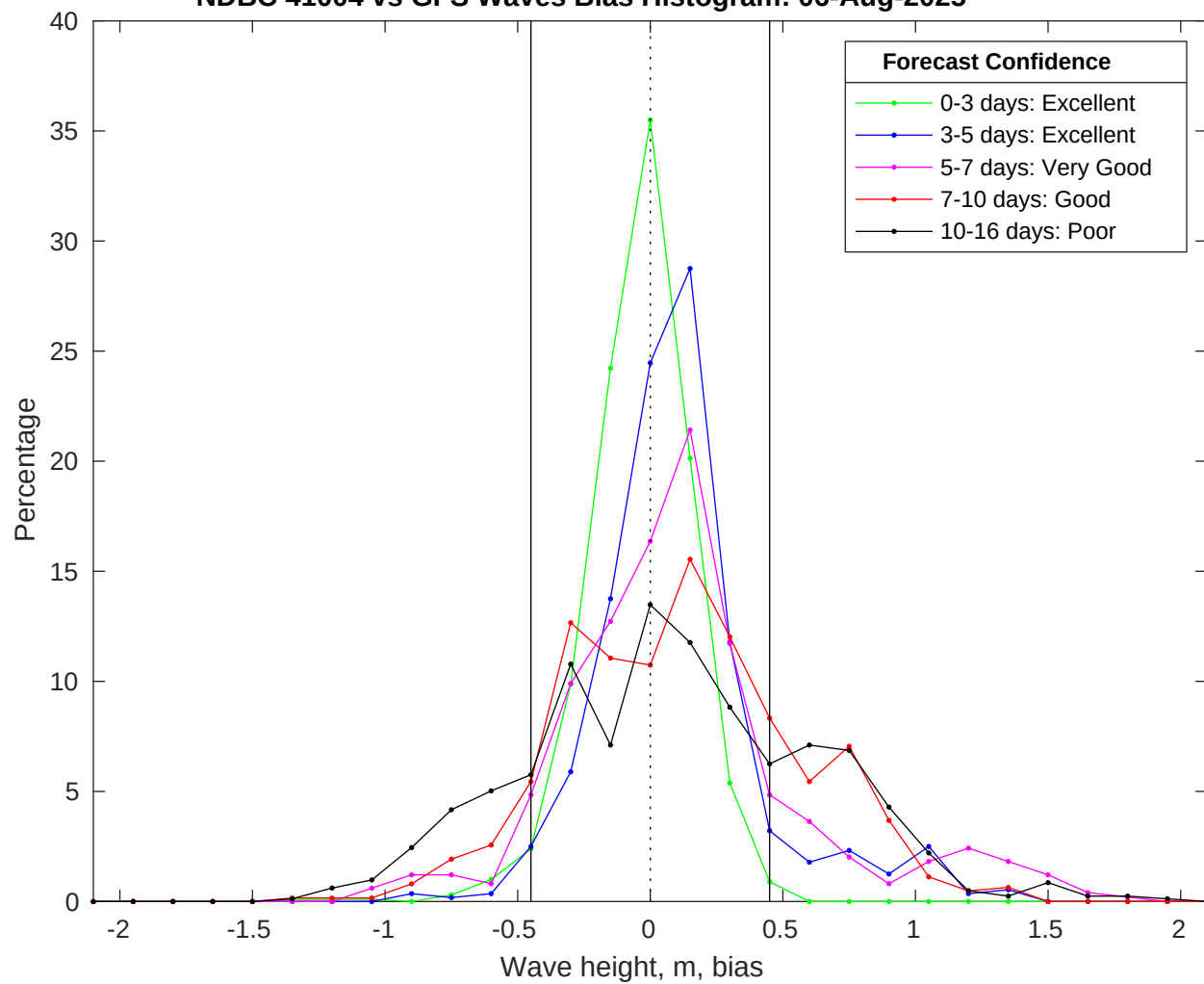
NDBC 41004 vs GFS Waves Bias Histogram: 06-Aug-2025
