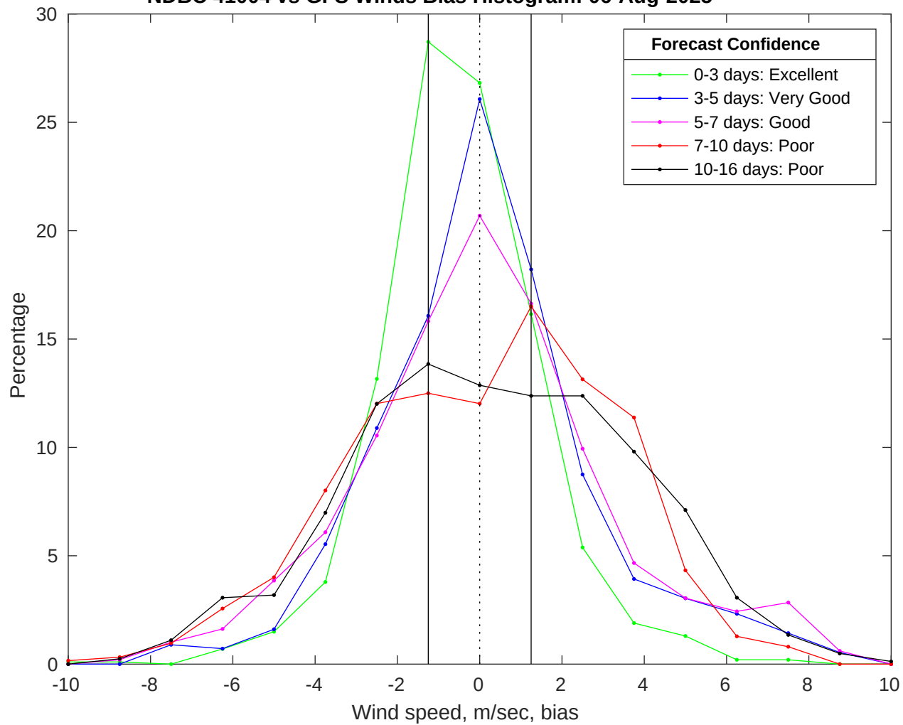
NDBC 41004 vs GFS Winds Bias Histogram: 06-Aug-2025
