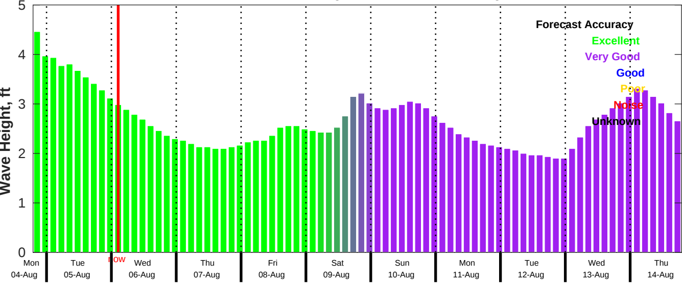
CMEMS Wave Forecast for NDBC 41004 from 04-Aug-2025 19:00:00 to 14-Aug-2025 19:00:00
