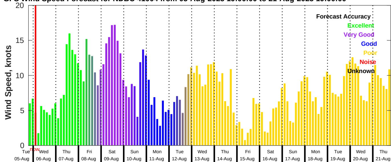
GFS Wind Speed Forecast for NDBC 41004 from 05-Aug-2025 19:00:00 to 21-Aug-2025 19:00:00
