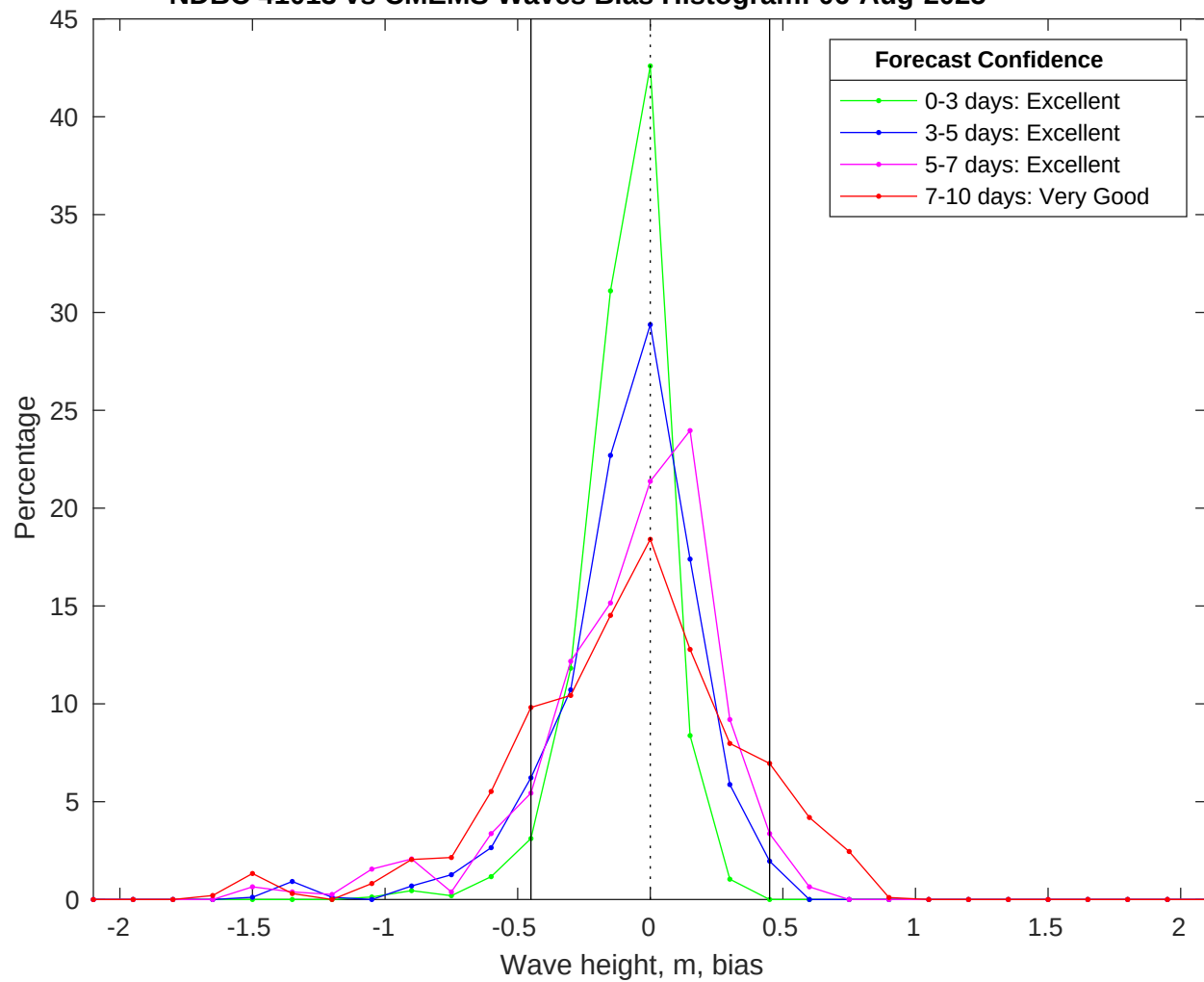
NDBC 41013 vs CMEMS Waves Bias Histogram: 06-Aug-2025
