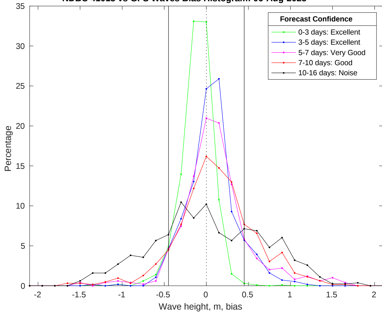
NDBC 41013 vs GFS Waves Bias Histogram: 06-Aug-2025
