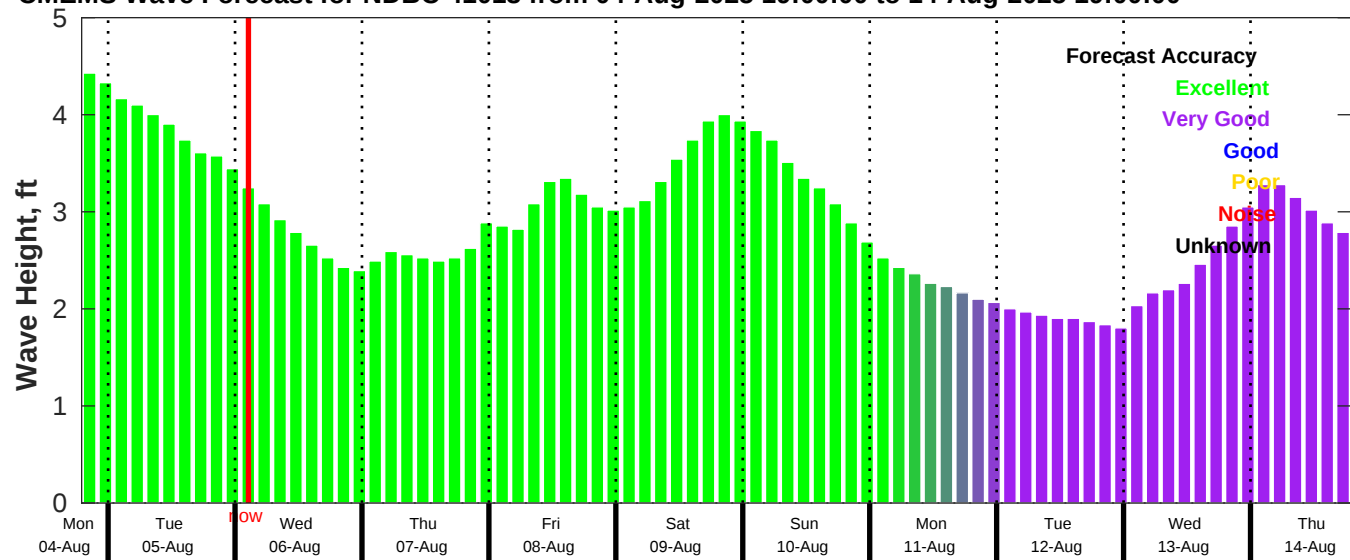
CMEMS Wave Forecast for NDBC 41013 from 04-Aug-2025 19:00:00 to 14-Aug-2025 19:00:00
