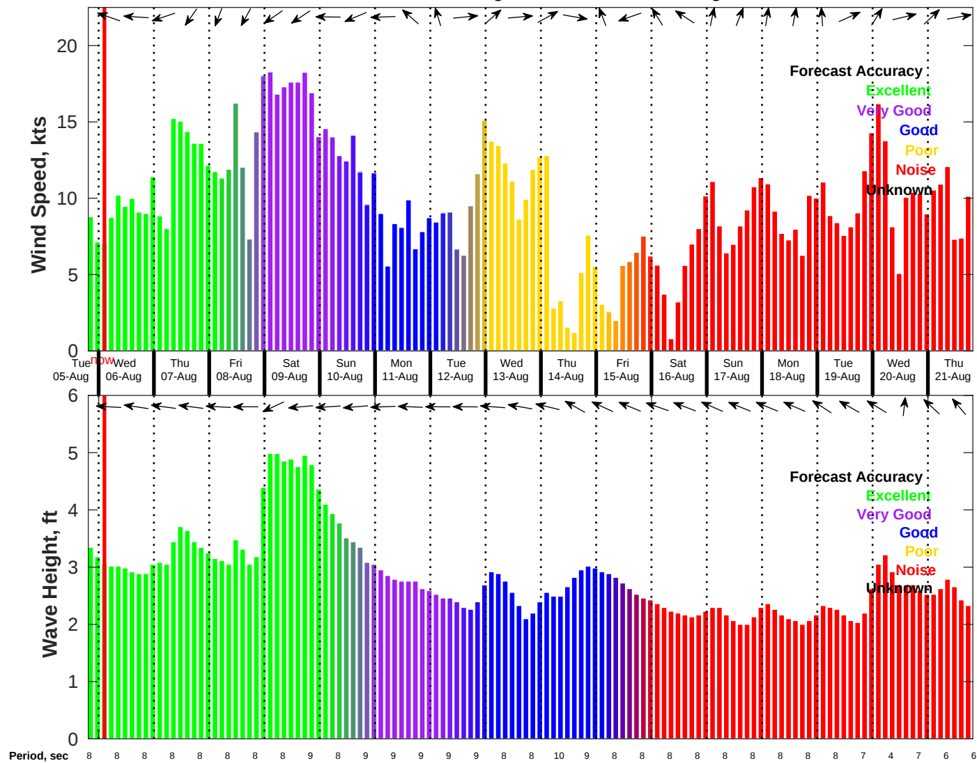
Wind & Wave Forecast for NDBC 41013 from 05-Aug-2025 19:00:00 to 21-Aug-2025 19:00:00
