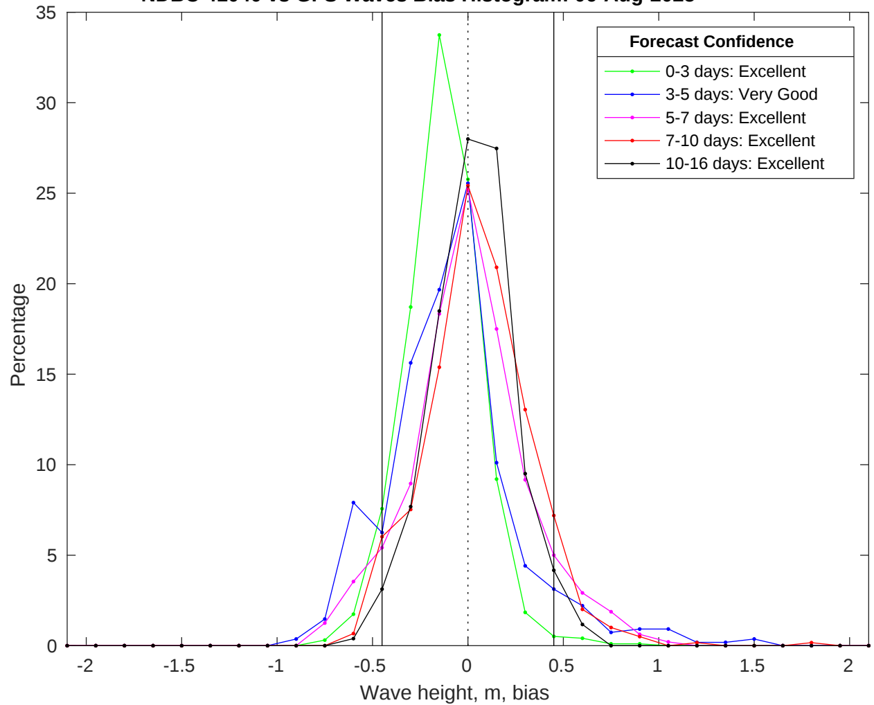
NDBC 41040 vs GFS Waves Bias Histogram: 06-Aug-2025
