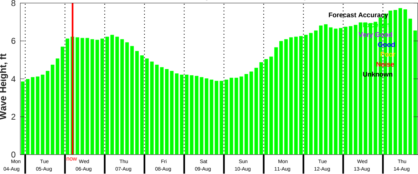
CMEMS Wave Forecast for NDBC 41040 from 04-Aug-2025 21:00:00 to 14-Aug-2025 21:00:00
