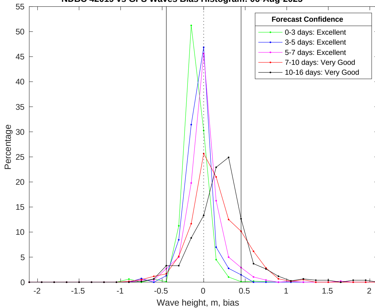
NDBC 42019 vs GFS Waves Bias Histogram: 06-Aug-2025
