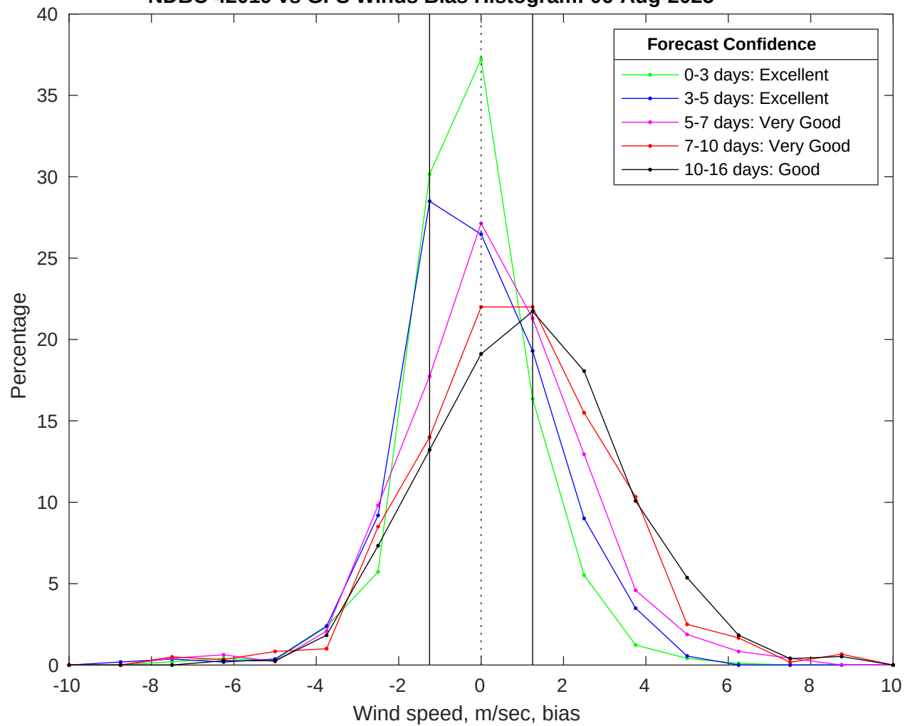
NDBC 42019 vs GFS Winds Bias Histogram: 06-Aug-2025
