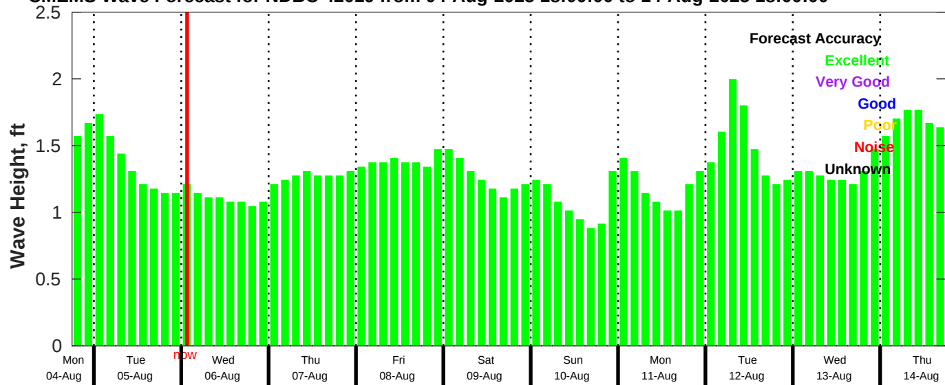
CMEMS Wave Forecast for NDBC 42019 from 04-Aug-2025 18:00:00 to 14-Aug-2025 18:00:00
