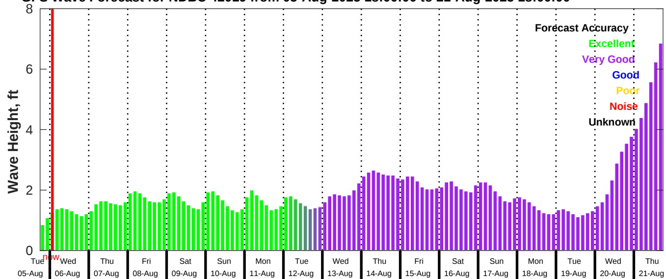
GFS Wave Forecast for NDBC 42019 from 05-Aug-2025 18:00:00 to 21-Aug-2025 18:00:00
