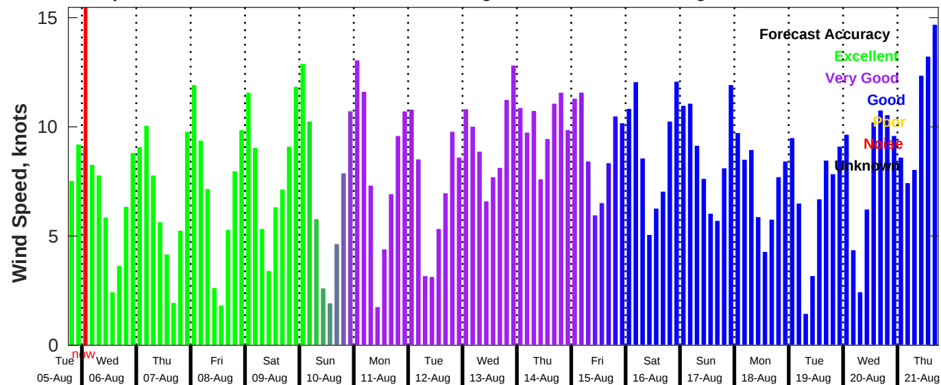
GFS Wind Speed Forecast for NDBC 42019 from 05-Aug-2025 18:00:00 to 21-Aug-2025 18:00:00
