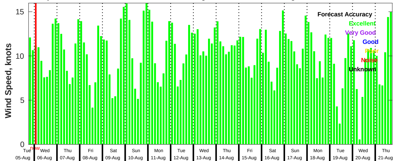
GFS Wind Speed Forecast for NDBC 42020 from 05-Aug-2025 18:00:00 to 21-Aug-2025 18:00:00
