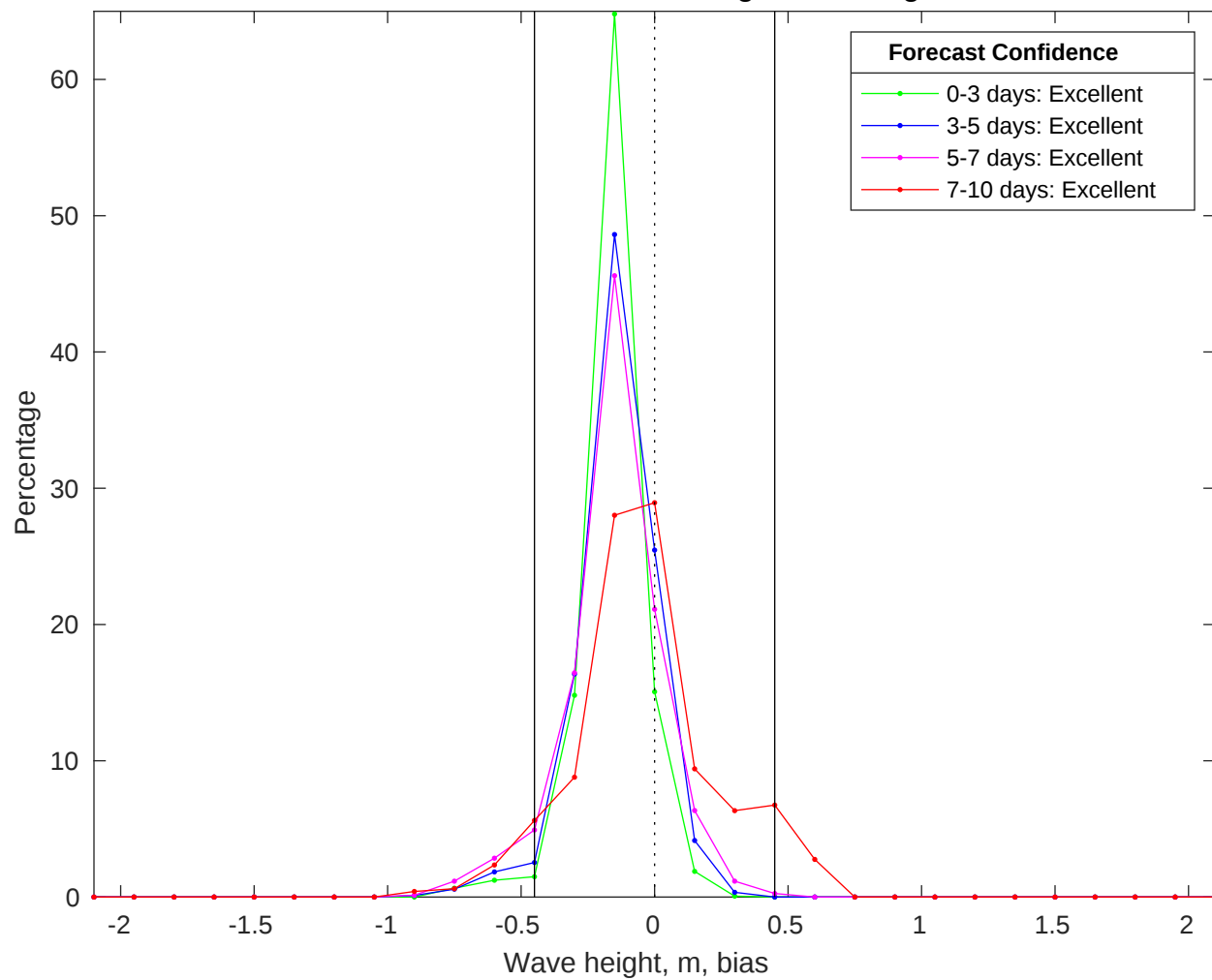
NDBC 42035 vs CMEMS Waves Bias Histogram: 06-Aug-2025
