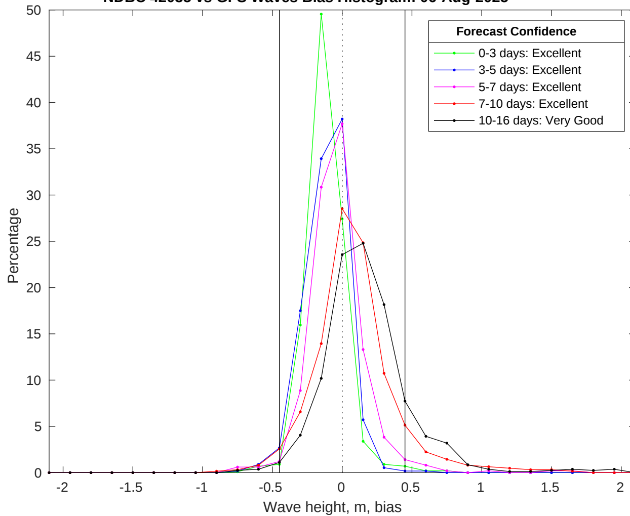
NDBC 42035 vs GFS Waves Bias Histogram: 06-Aug-2025
