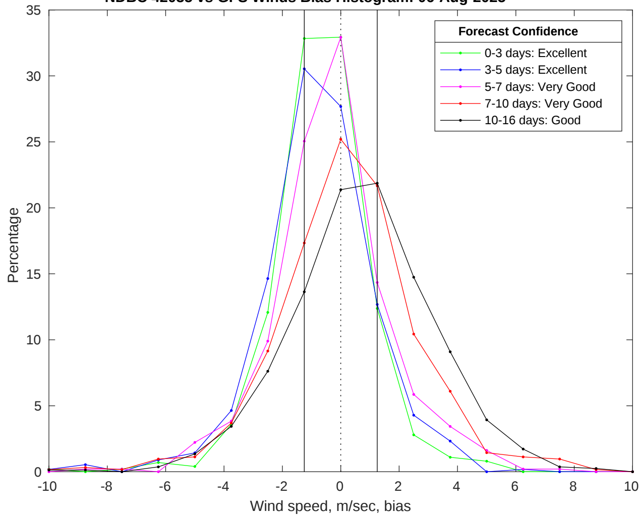
NDBC 42035 vs GFS Winds Bias Histogram: 06-Aug-2025
