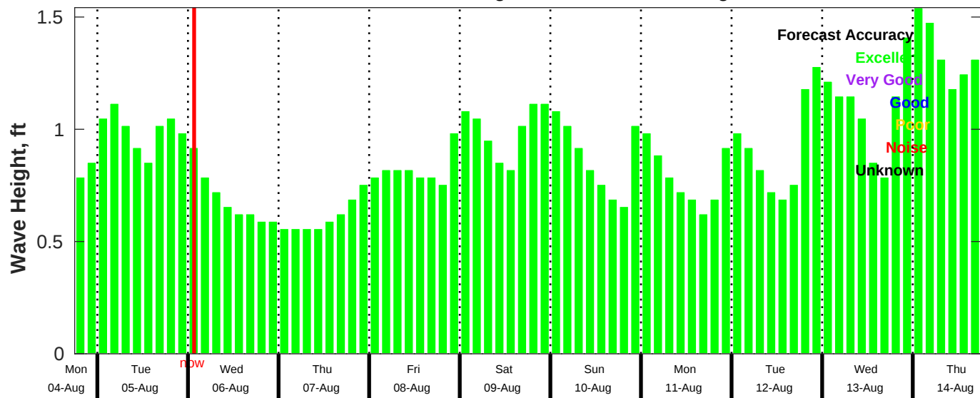
CMEMS Wave Forecast for NDBC 42035 from 04-Aug-2025 18:00:00 to 14-Aug-2025 18:00:00
