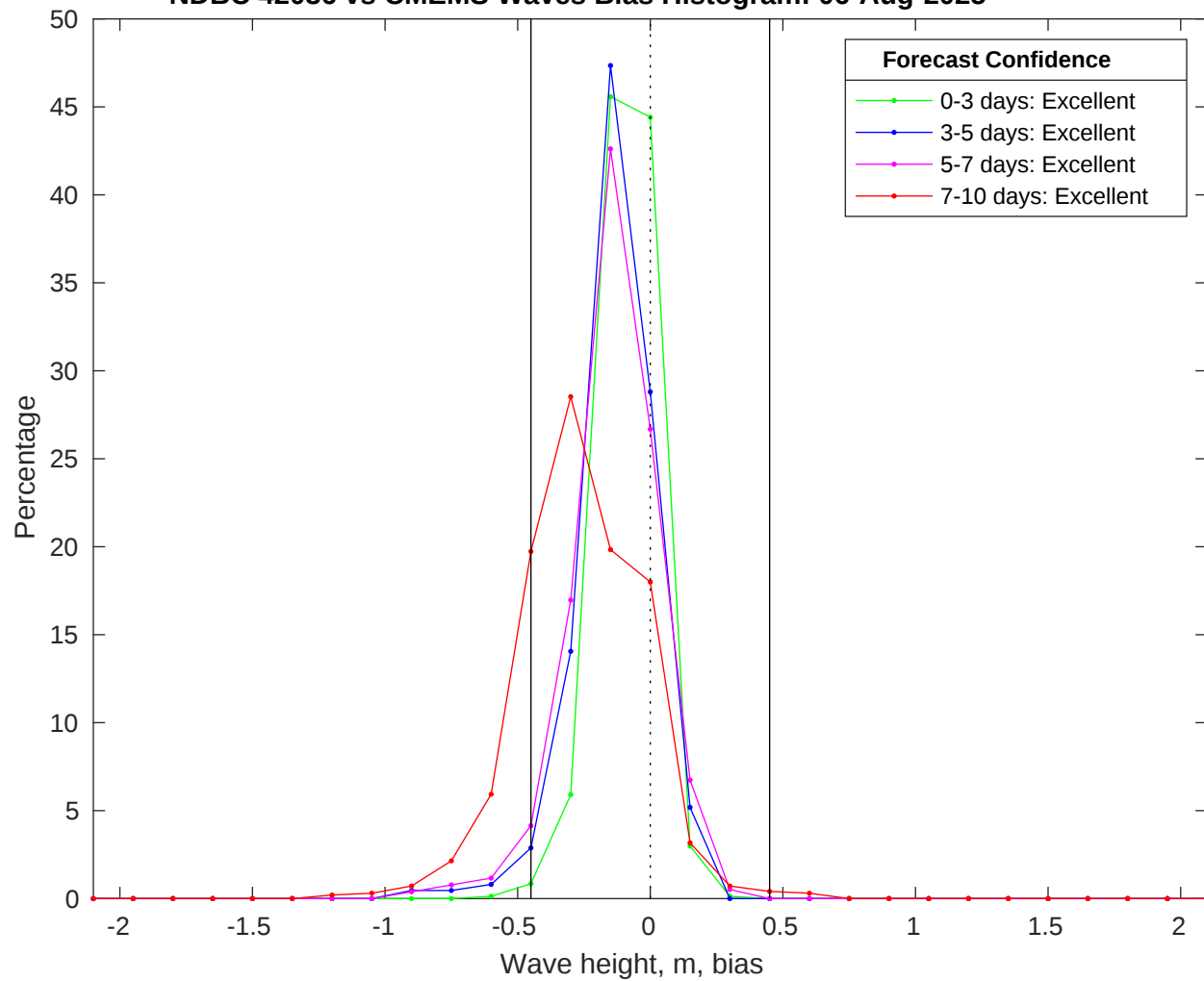
NDBC 42036 vs CMEMS Waves Bias Histogram: 06-Aug-2025
