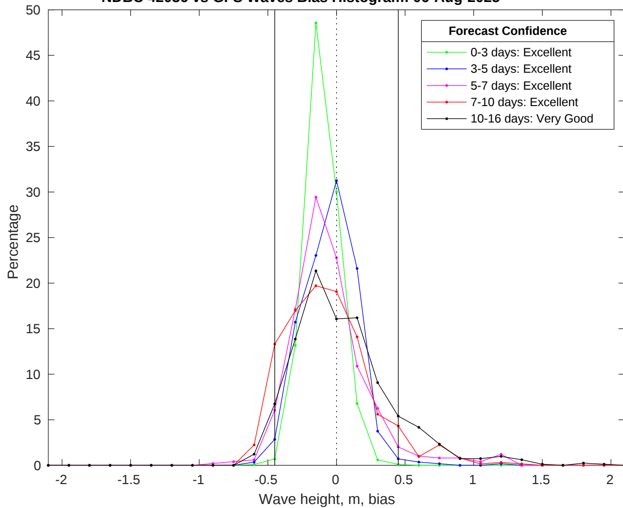
NDBC 42036 vs GFS Waves Bias Histogram: 06-Aug-2025
