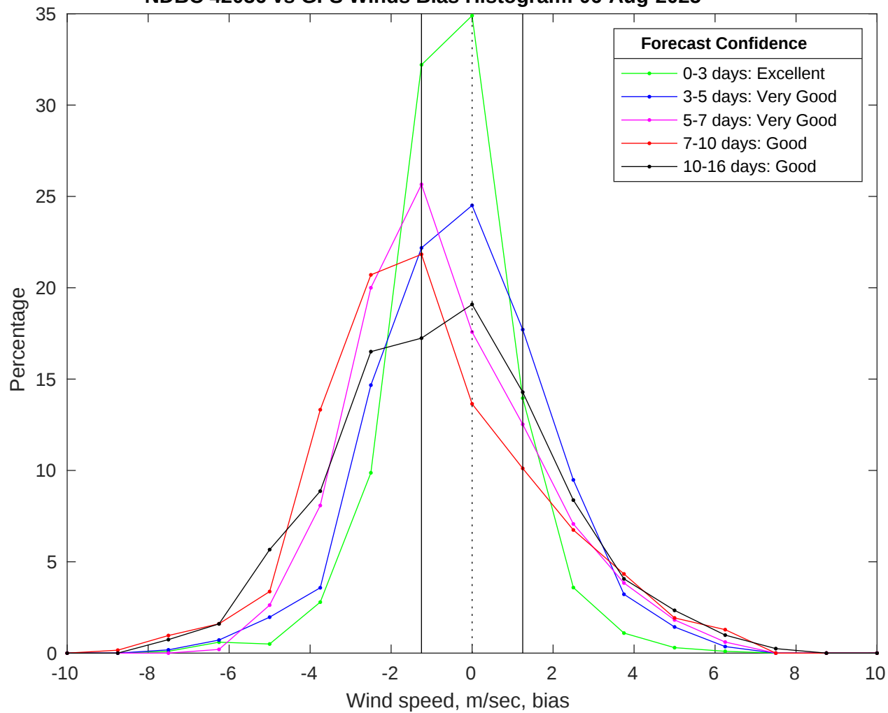
NDBC 42036 vs GFS Winds Bias Histogram: 06-Aug-2025
