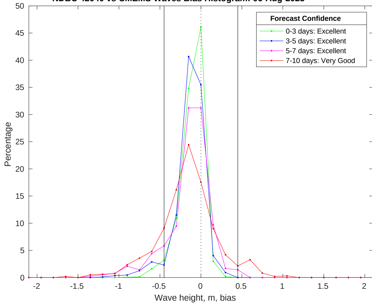
NDBC 42040 vs CMEMS Waves Bias Histogram: 06-Aug-2025
