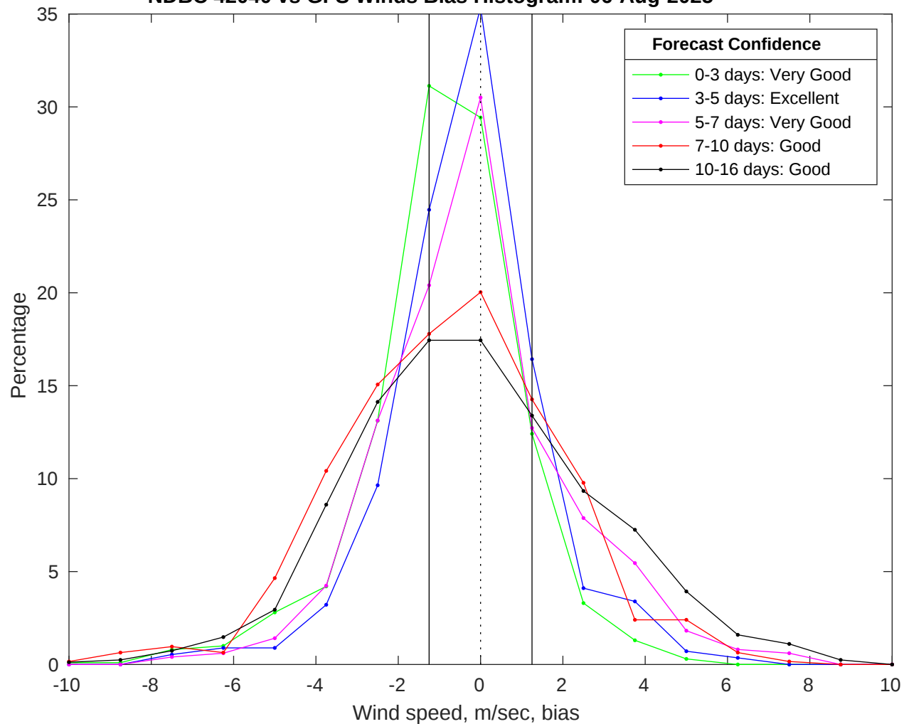
NDBC 42040 vs GFS Winds Bias Histogram: 06-Aug-2025
