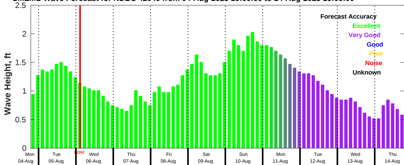
CMEMS Wave Forecast for NDBC 42040 from 04-Aug-2025 19:00:00 to 14-Aug-2025 19:00:00
