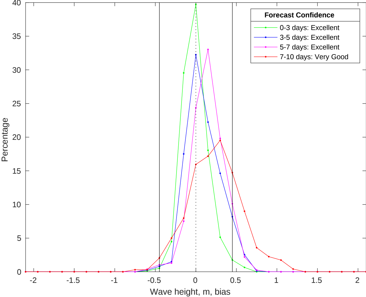
NDBC 46011 vs CMEMS Waves Bias Histogram: 06-Aug-2025
