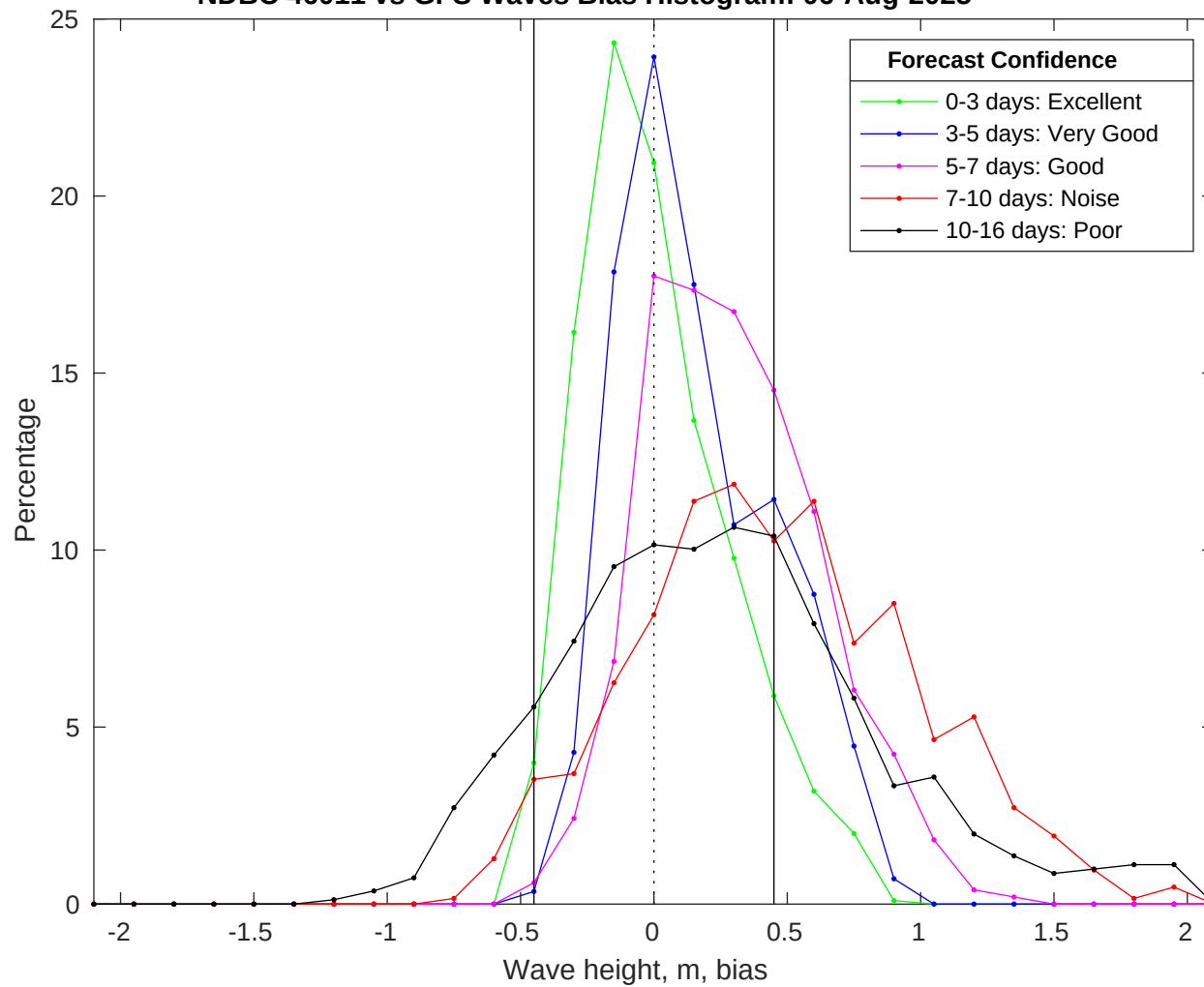
NDBC 46011 vs GFS Waves Bias Histogram: 06-Aug-2025
