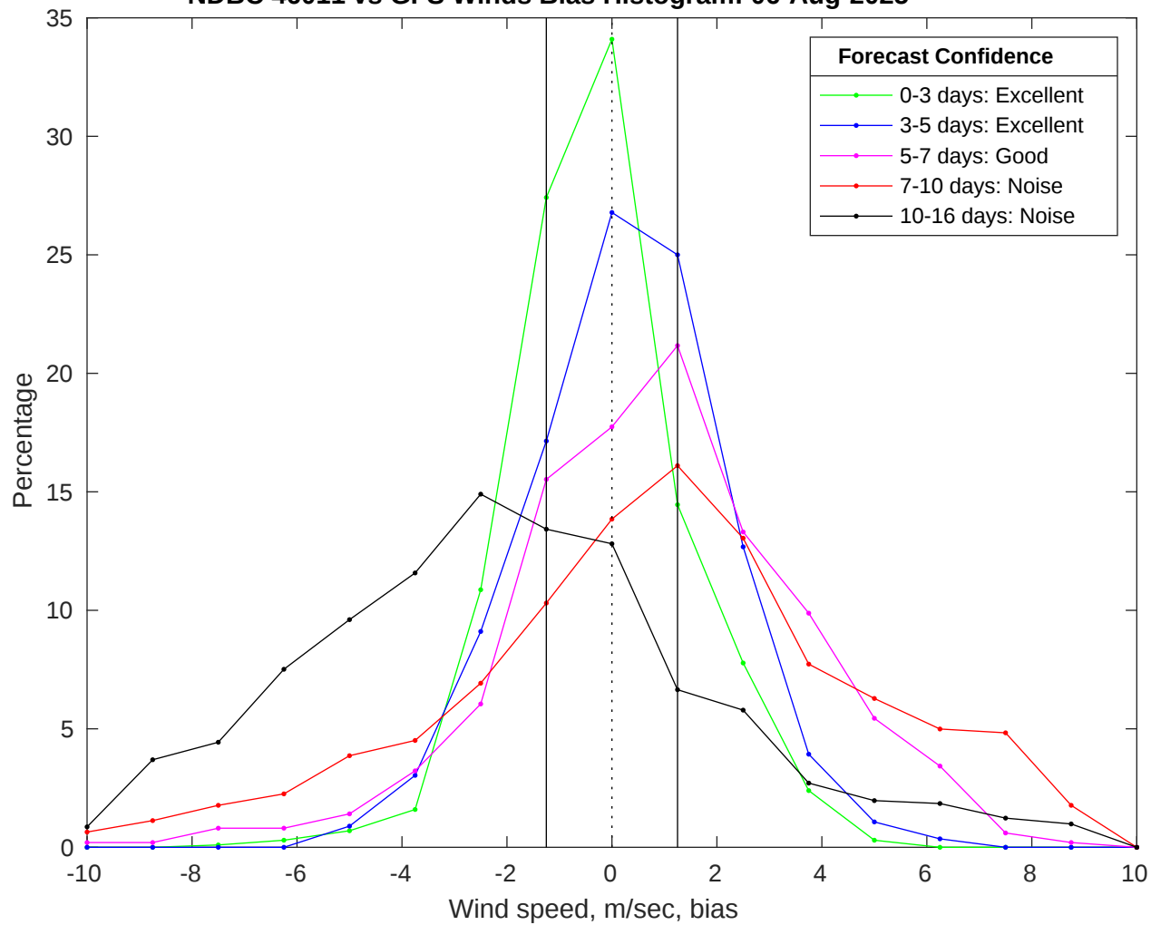
NDBC 46011 vs GFS Winds Bias Histogram: 06-Aug-2025
