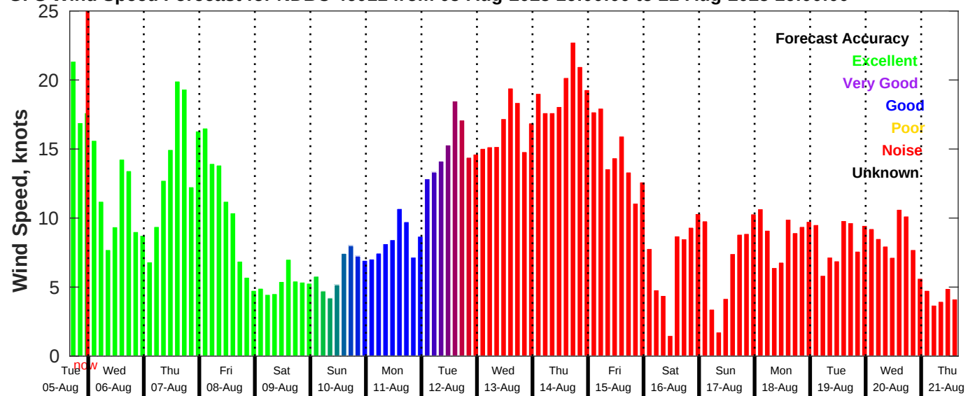
GFS Wind Speed Forecast for NDBC 46011 from 05-Aug-2025 16:00:00 to 21-Aug-2025 16:00:00
