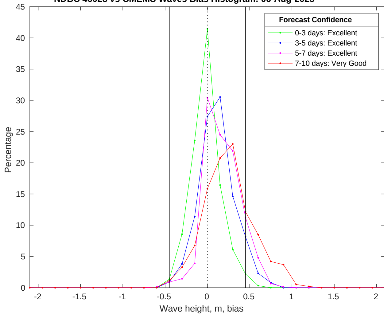
NDBC 46028 vs CMEMS Waves Bias Histogram: 06-Aug-2025
