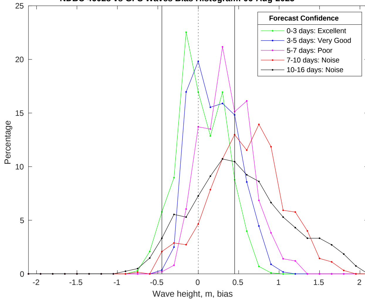
NDBC 46028 vs GFS Waves Bias Histogram: 06-Aug-2025
