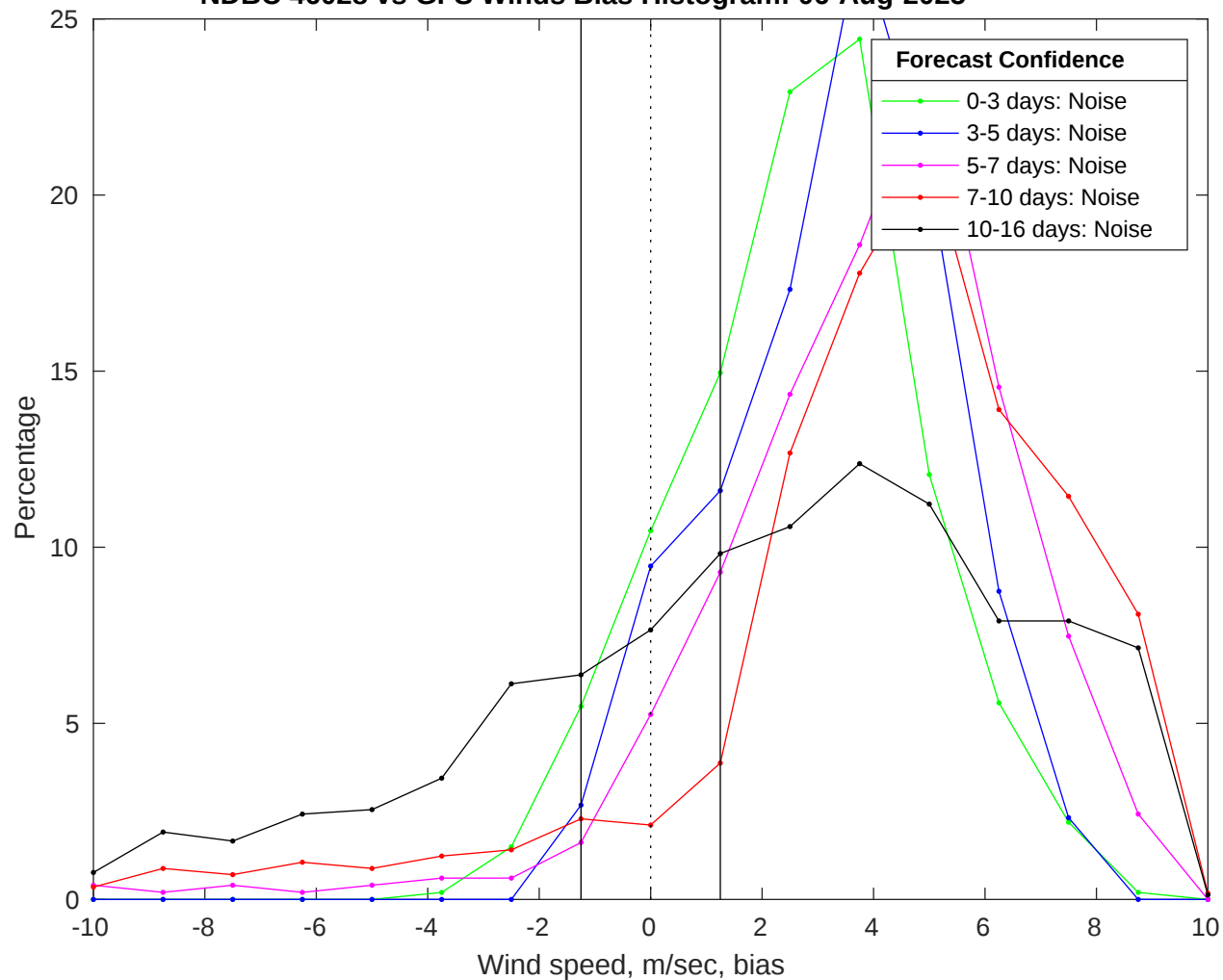
NDBC 46028 vs GFS Winds Bias Histogram: 06-Aug-2025
