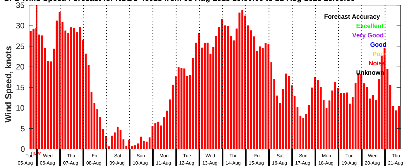
GFS Wind Speed Forecast for NDBC 46028 from 05-Aug-2025 16:00:00 to 21-Aug-2025 16:00:00
