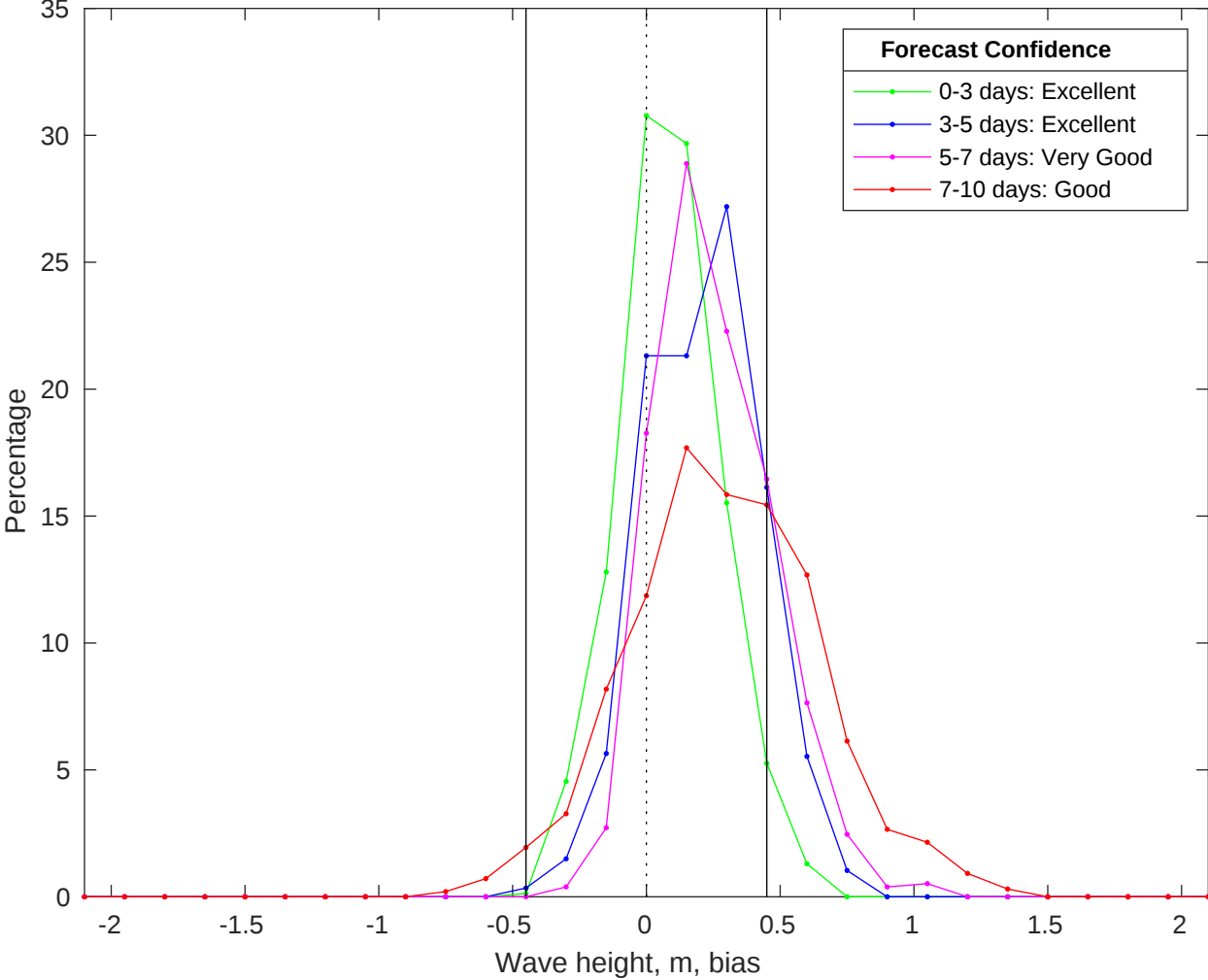
NDBC 46054 vs CMEMS Waves Bias Histogram: 06-Aug-2025
