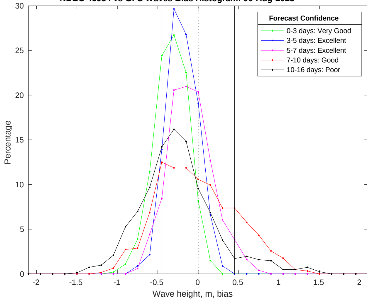
NDBC 46054 vs GFS Waves Bias Histogram: 06-Aug-2025
