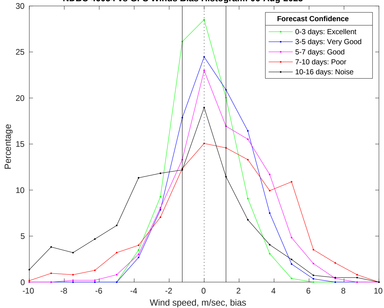
NDBC 46054 vs GFS Winds Bias Histogram: 06-Aug-2025
