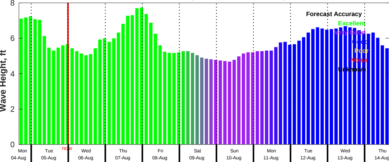
CMEMS Wave Forecast for NDBC 46054 from 04-Aug-2025 16:00:00 to 14-Aug-2025 16:00:00
