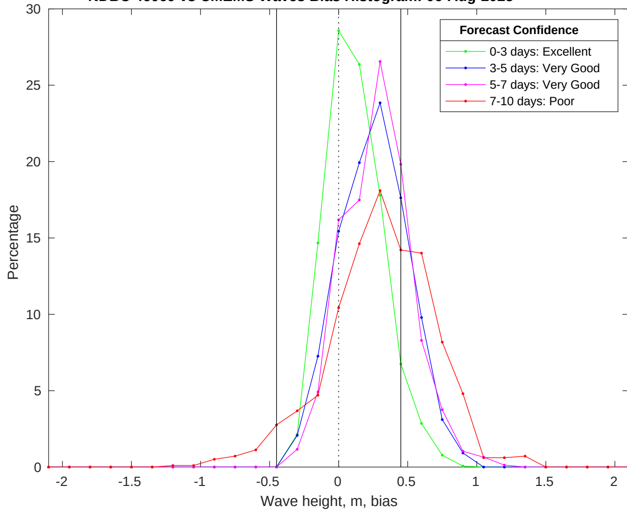
NDBC 46069 vs CMEMS Waves Bias Histogram: 06-Aug-2025
