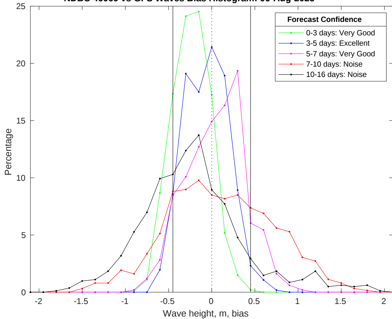
NDBC 46069 vs GFS Waves Bias Histogram: 06-Aug-2025
